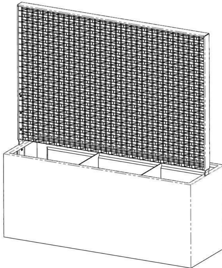
Centered Trellis Shown (offset optional, same assembly procedure)
